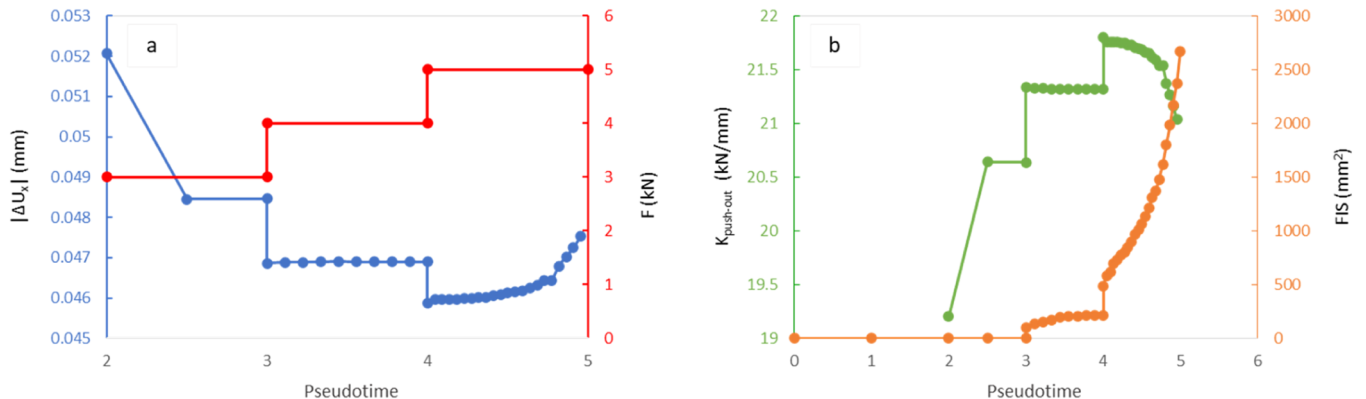
Fig. 7. a) Relative displacement of the node where the load was applied during the push-out test (in blue) plotted against pseudotime. The compressive load applied is also depicted in the graph (in red). b) Push-out stiffness (in green) and Fracture Internal Surface (in orange) curves plotted against pseudotime.
