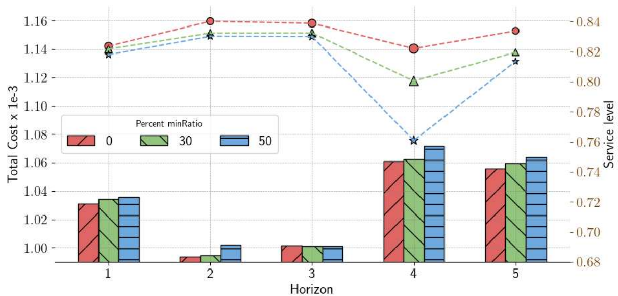
Figure 11: Rolling horizon results for comparing minimum ratio values.
