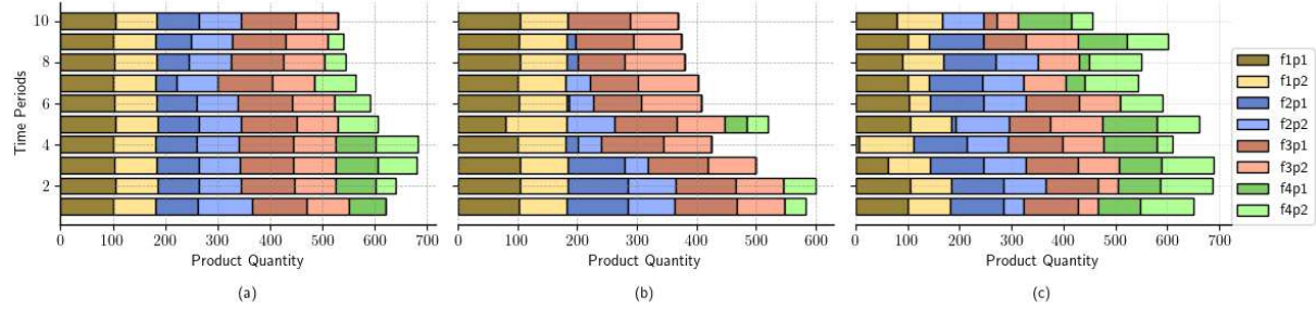
Figure 5: Aggregated scheduling profile for objectives (a) Cost; (b) Env. Impact; (c) Max Ratio
