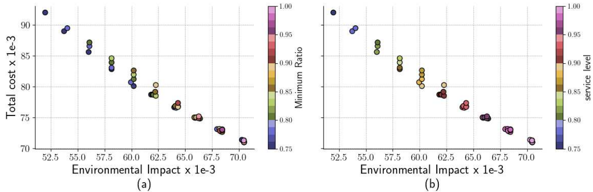
Figure 6: Pareto Frontier for Case I: (a) Total cost vs Environmental Impact with minimum ratio ; (b) Total cost vs Environmental Impact with service level.
