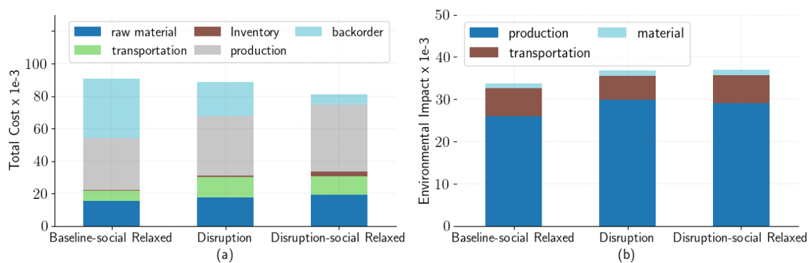
Figure 9: Objective distribution for all models; (a) Cost Distribution; (b) Environmental Distribution
