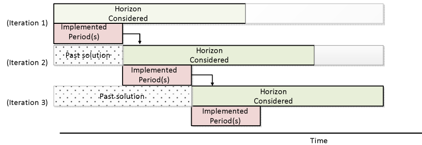
Figure 2: Rolling Horizon Framework
