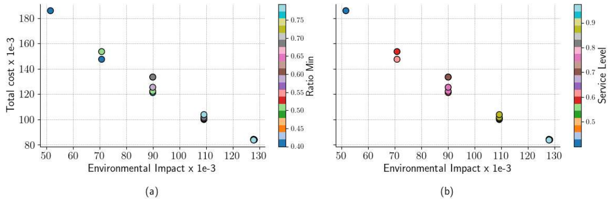
Figure 7: Pareto Frontier for Case II: (a) Total cost vs Environmental Impact with minimum ratio; (b) Total cost vs Environmental Impact with service level.
