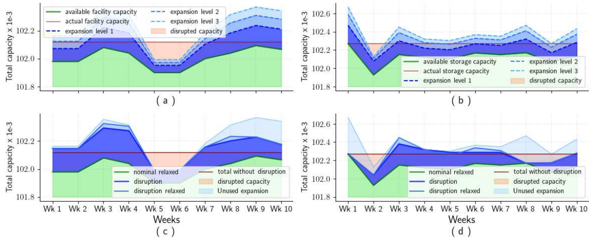
Figure 8: Capacity profile for manufacturing facility and warehouses. (a) available capacity and the expansion levels at manufacturing facility; (b) available capacity and the expansion levels at warehouses; (c) comparison of capacity levels used by the models for manufacturing sites; (d) comparison of capacity levels used by the models for warehouses.
