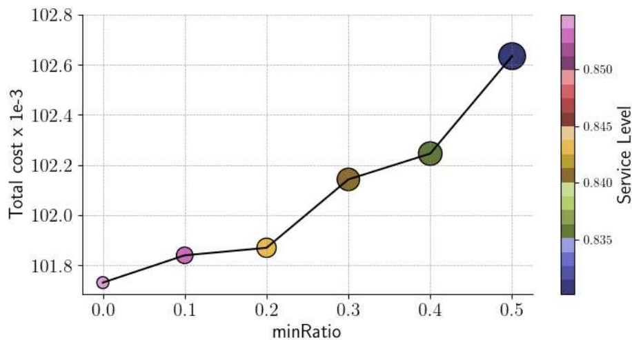
Figure 10: Cost against minimum ratio.
