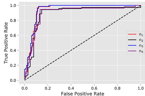
(b) ROC Curve of S_2
