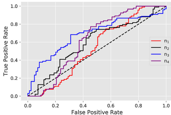
(a) ROC Curve of S_1
