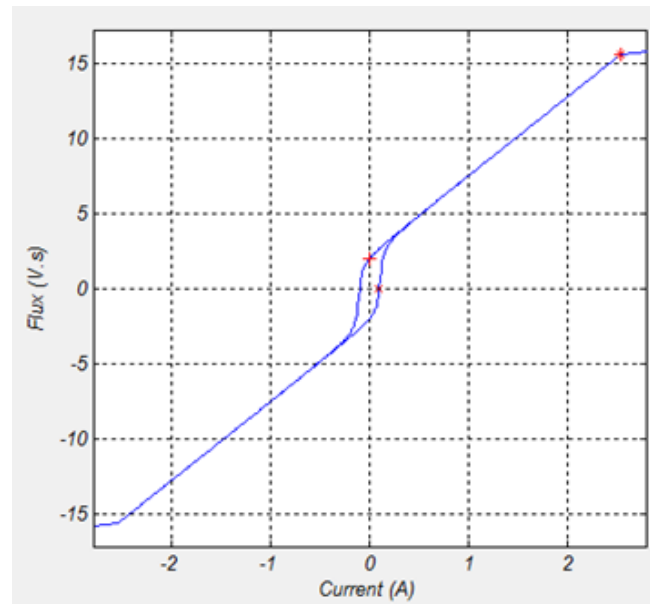
Fig. 2. Hysteresis characteristics.
