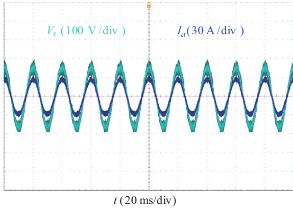
Fig. 19. Grid-side current and voltage.
