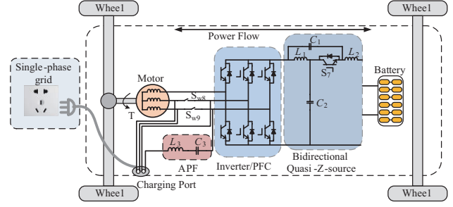
Fig. 14. Proposed single-phase integrated charger .
