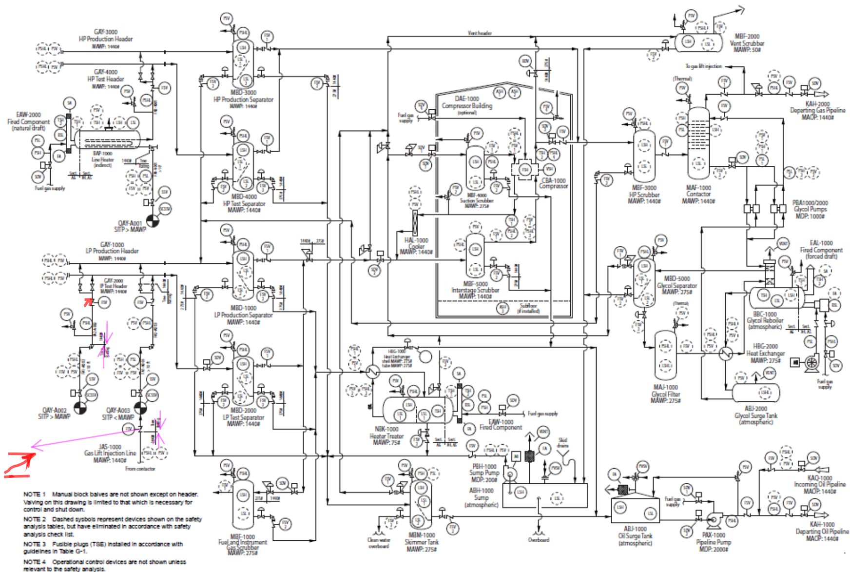
Figure B.1—Example Safety Analysis Flow Diagram of Platform Production Process
