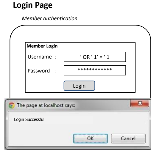
Figure 12. Before applying encryption algorithm
