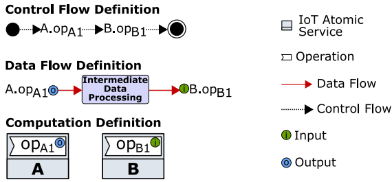
Fig. 12. Separation of control, data and computation.
