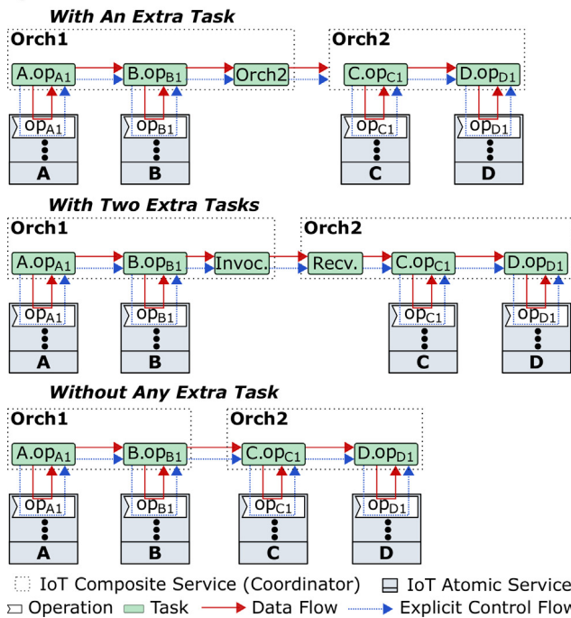
Fig. 16. Composition by orchestration.
