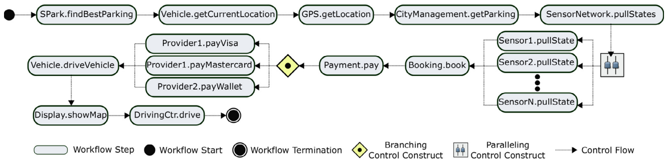
Fig. B.1. SPark workflow control flow.
