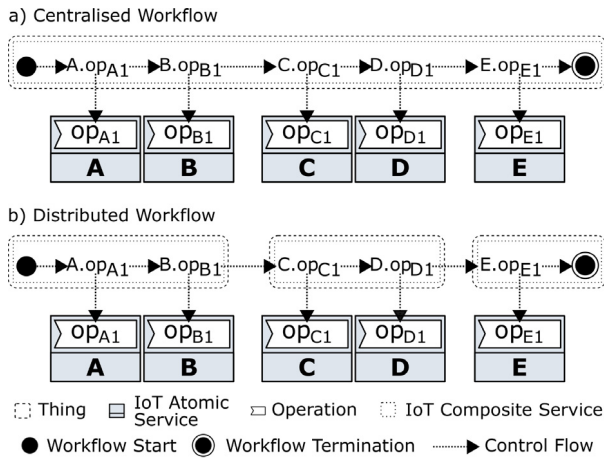
Fig. 10. Centralised workflow vs distributed workflow.
