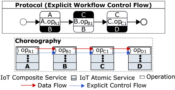
Fig. 17. Composition by choreography.
