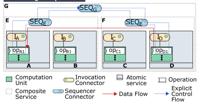
Fig. 22. A workflow variant derived from Fig. 20 for sequentially executing D.op_{D1} and A.op_{A1} .
