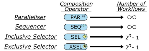
Fig. 19. DX-MAN composition operators.
