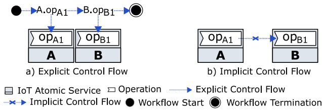
Fig. 8. Explicit control flow vs implicit control flow.
