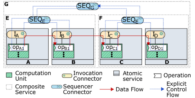
Fig. 21. A workflow variant derived from Fig. 20 for sequentially executing A.op_{A1} , B.op_{B1} , C.op_{C1} and D.op_{D1} .
