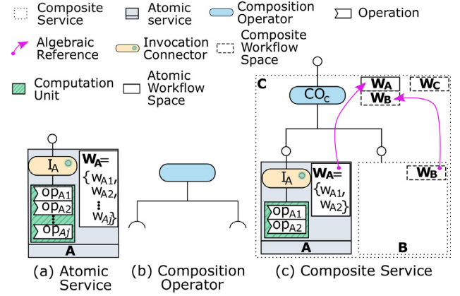
Fig. 18. DX-MAN model.
