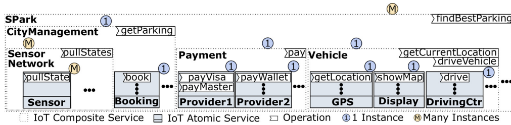
Fig. 7. SPark services.
