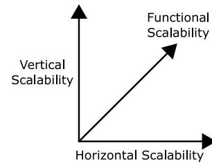
Fig. 4. Scalability dimensions.
