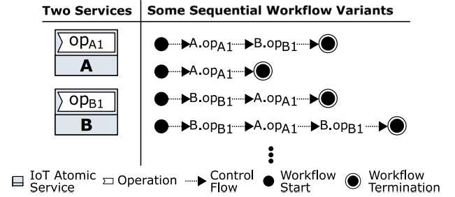
Fig. 13. Workflow variability.
