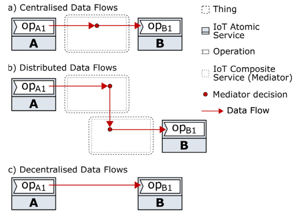
Fig. 11. Data flow approaches.
