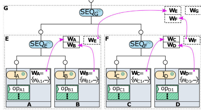
Fig. 21. A workflow variant derived from Fig. 20 for sequentially executing A.op_{A1} , B.op_{B1} , C.op_{C1} and D.op_{D1} .
