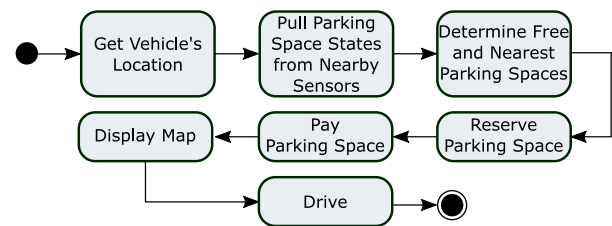
Fig. 6. SPark workflow.
