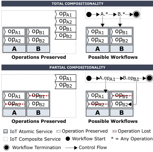
Fig. 14. Total compositionality vs partial compositionality.
