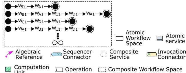
Fig. 20. Composition by DX-MAN.
