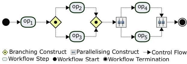
Fig. 2. A generic workflow.
