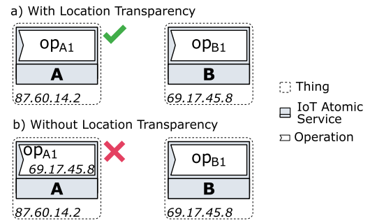
Fig. 9. Location transparency.
