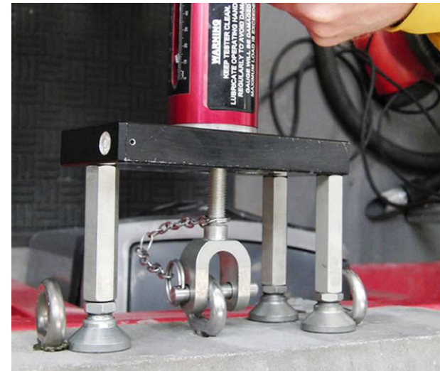
Mechanical components for Anchor wire rope pull out test
