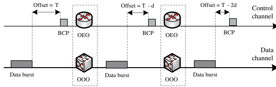
Figure 1. Offset time is gradually reduced as it passes each hop.
