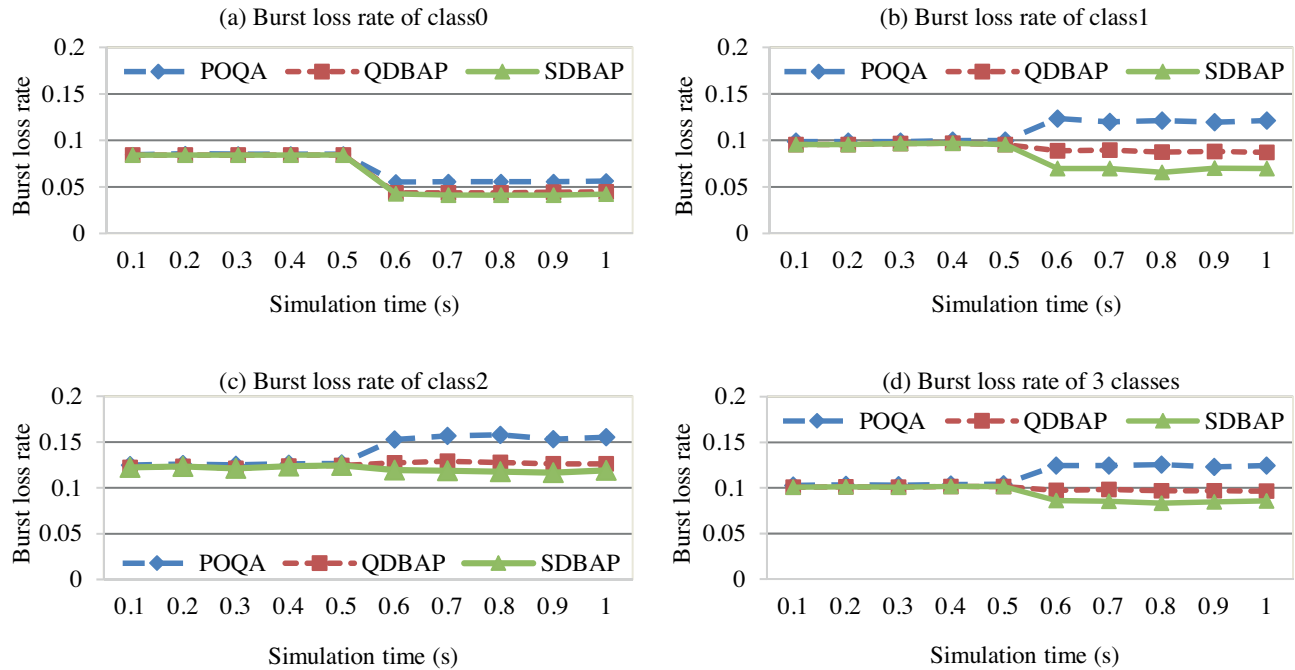
Figure 10. Comparison of the burst loss rate of each class and all 3 classes between POQA, QDBAP and SDBAP.
