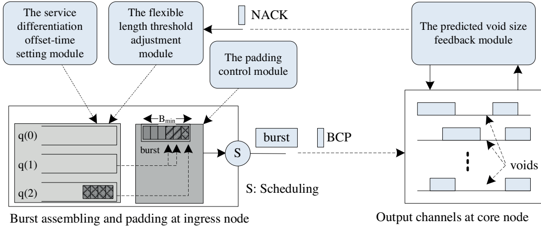
Figure 6. The model of service differentiation burst assembly and padding.
