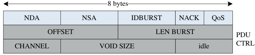
Figure 8. The modified structure of NACK packet with 4 bytes dedicated to carry the predicted void size.
