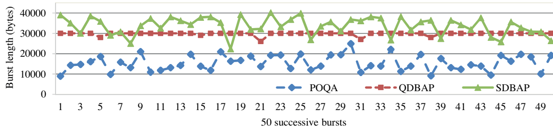
Figure 13. Comparison of the length of 50 consecutive completed bursts between POQA, QDBAP and SDBAP.
