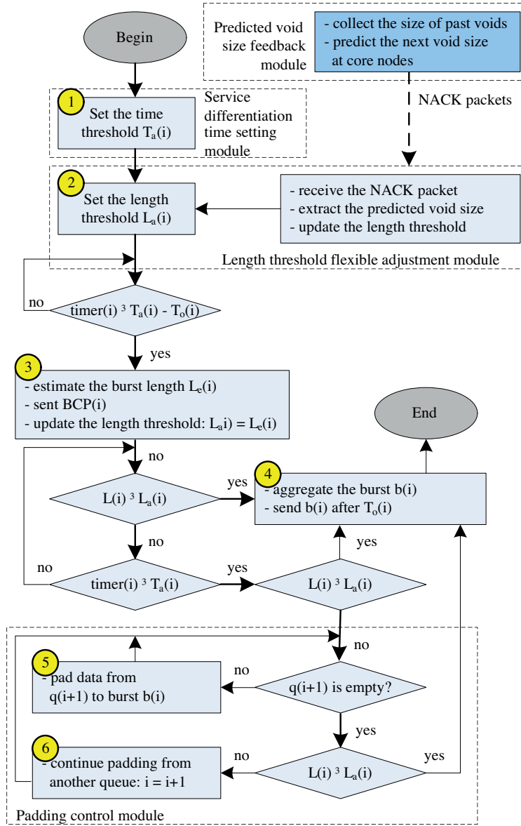
Figure 9. The algorithm of service differentiation burst assembly and padding.
