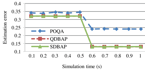
Figure 15. Comparison of the estimation error between POQA, QDBAP and SDBAP.
