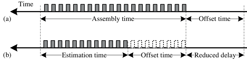
Figure 3. Solution of nesting the offset time into the assembly time to reduce transmission delay.
