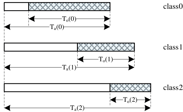
Figure 4. An example of the different assembly times and offset times for service differentiation.
