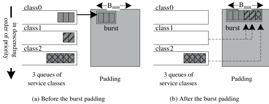
Figure 5. An example of the burst padding method with 3 classes: (a) before padding and (b) after padding.
