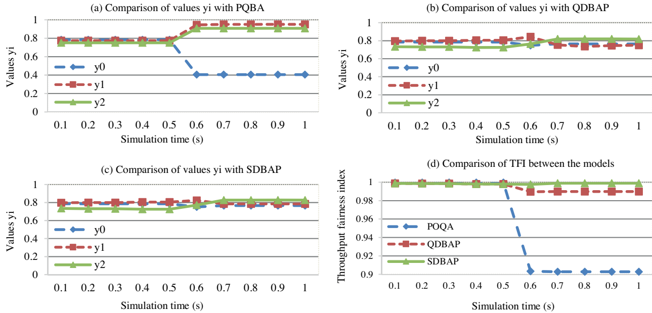
Figure 14. Comparison of the throughput fairness between POQA, QDBAP and SDBAP.
