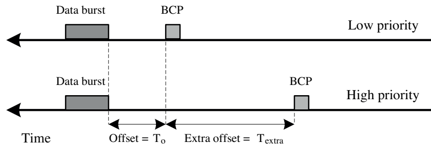
Figure 2. Offset time-based service differentiation scheme.
