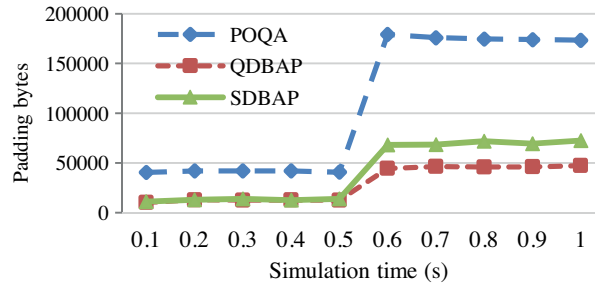
Figure 12. Comparison of the padding bytes between POQA, QDBAP and SDBAP.
