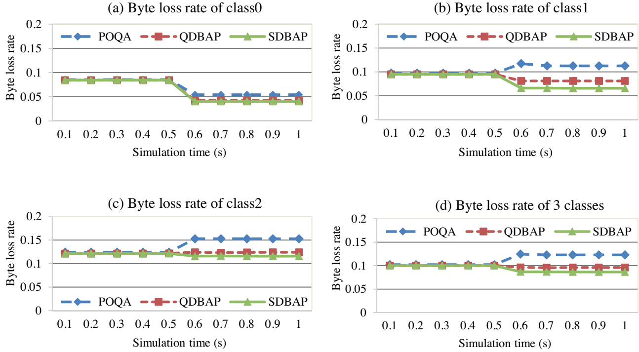
Figure 11. Comparison of the byte loss rate of each class and all 3 classes between POQA, QDBAP and SDBAP.
