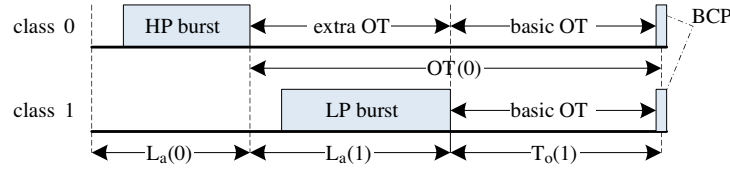
Figure 7. The offset time of the high-priority burst must be greater than the sum of the offset time and the length of the low-priority burst.
