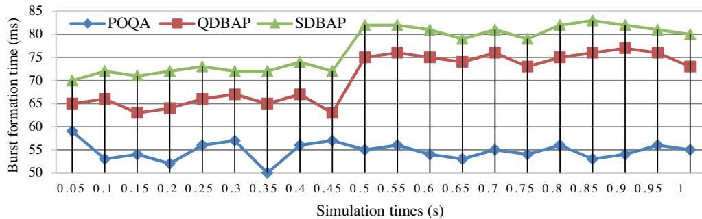
Figure 16. Comparison of the average burst formation time between POQA, QDBAP and SDBAP.
