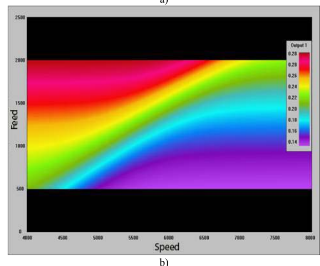
Fig. 3: Effects of feed rate and speed on the R_a (finishing). a) via RSM, b) via ANN
