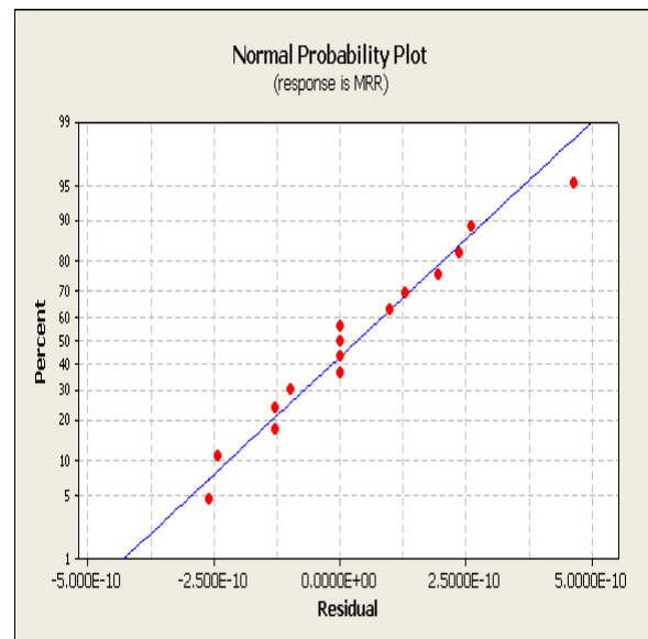
Fig. 6-b: Residual distribution of MRR (rough machining)
