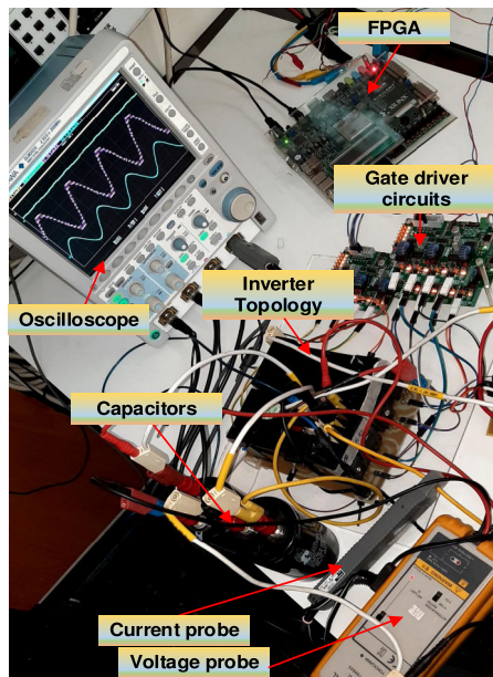
FIGURE 7. Experimental Setup.
