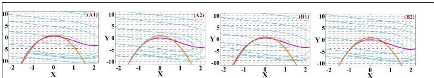
Fig. 4. Dynamics of the HR neuron model. (A1)-(A2): Dynamical behaviors of the original HR model for I = 0.5 and I = 1 . (B1)-(B2): Dynamical behaviors of the proposed N-LUT-HR model for I = 0.5 and I = 1 .
