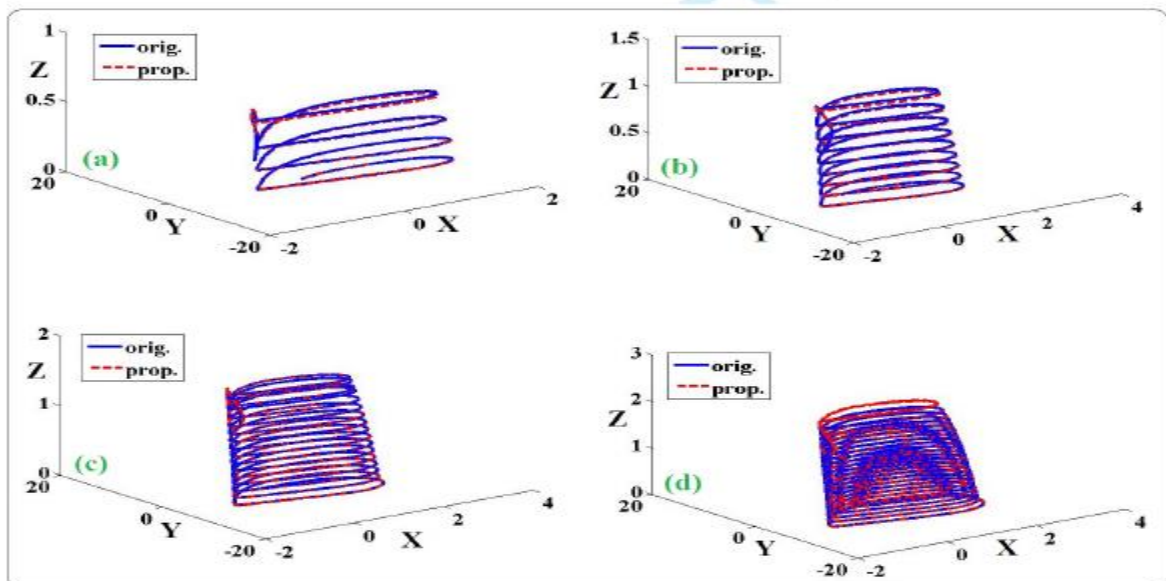
Fig. 5. Representation of the phase portraits in two models. (a) Phase portraits of two models for I_{\text{stimulus}} = 0.5 . (b) Phase portraits of two models for I_{\text{stimulus}} = 1 . (c) Phase portraits of two models for I_{\text{stimulus}} = 1.5 . (d) Phase portraits of two models for I_{\text{stimulus}} = 2 .
